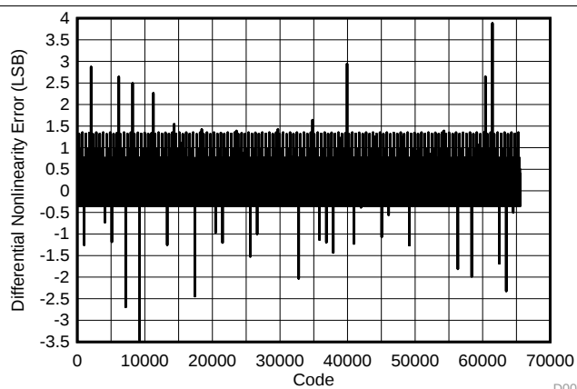
Figure 2. Differential Nonlinearity
