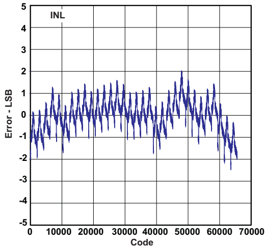
Figure 1. Integral Non-Linearity
