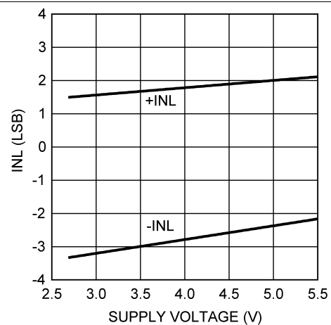
Figure 7. INL vs V_A
