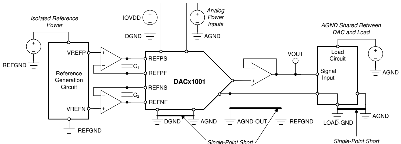
Figure 73. Grounding Scheme When AGND is Load Ground
