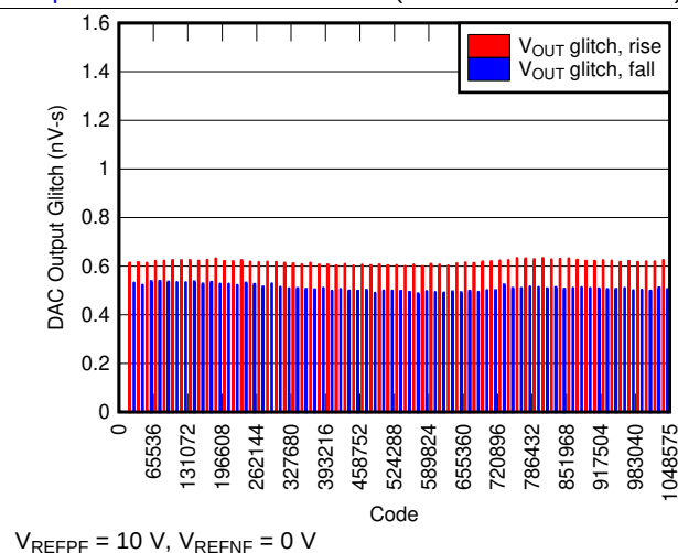
Figure 34. Segment Glitch Impulse, 1-LSB Step
