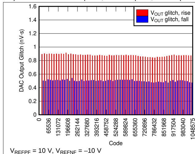
Figure 33. Segment Glitch Impulse, 1-LSB Step
