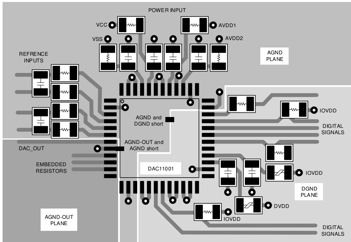
Figure 77. Layout Example
