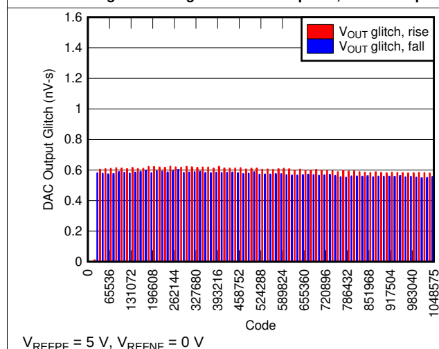
Figure 35. Segment Glitch Impulse, 1-LSB Step
