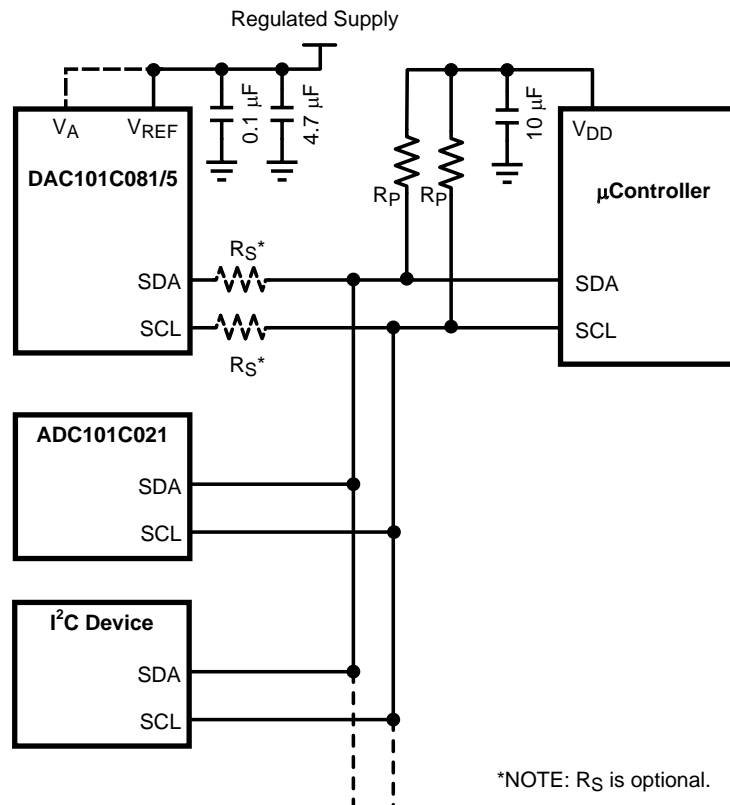
Figure 28. Serial Interface Connection Diagram
