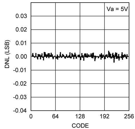
Figure 5. DNL
