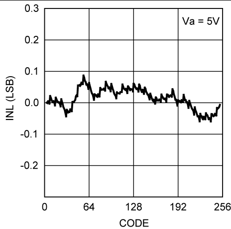
Figure 4. INL
