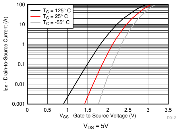
Figure 4-9. MOSFET Transfer Characteristics
