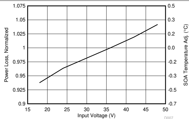
Figure 4-5. Normalized Power Loss vs Input Voltage
