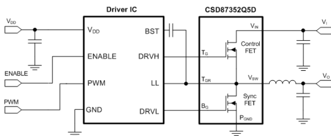
Typical Circuit
