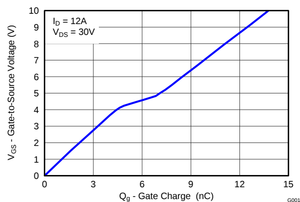
Gate Charge
