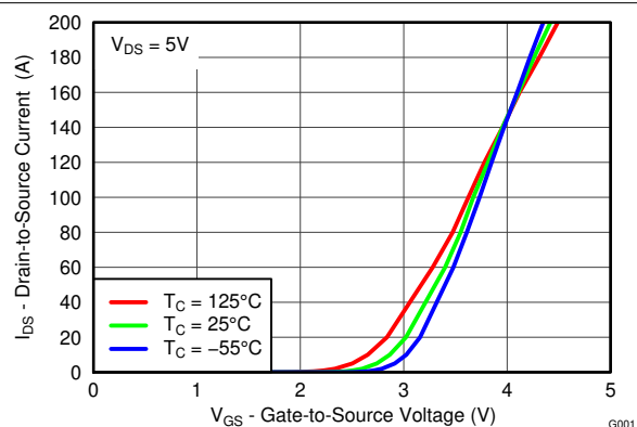
Figure 4-3. Transfer Characteristics
