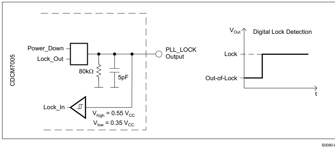
Figure 18. Digital Lock-Detect
