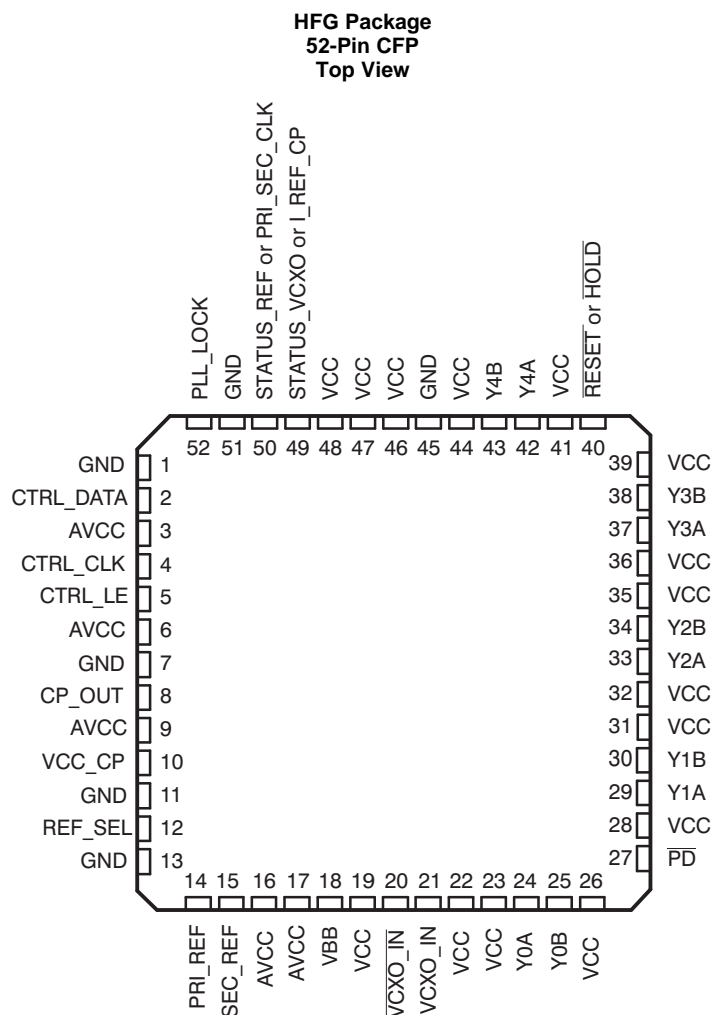
Pin Functions
