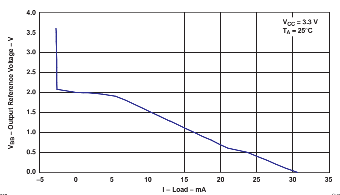
Figure 9. Output Reference Voltage (VBB) vs Load
