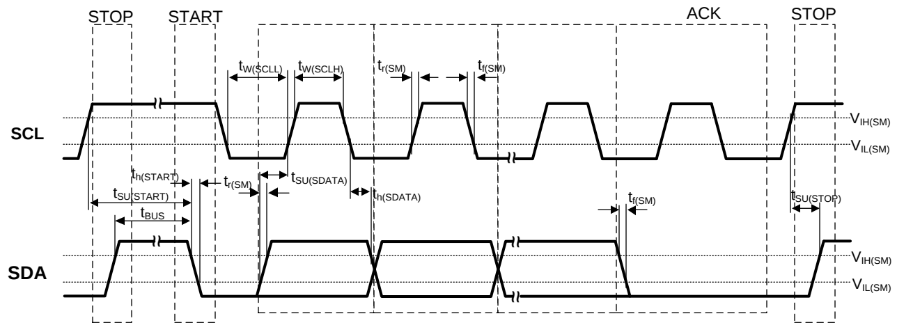
Figure 2. I²C Timing Diagram
