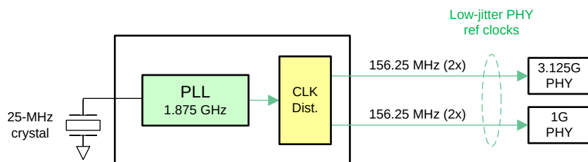
Figure 23. Ethernet Switch
