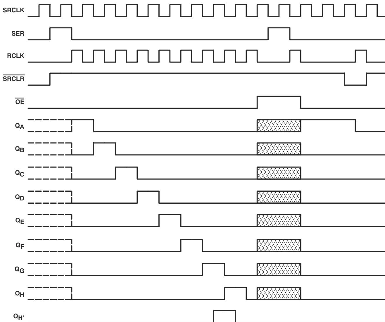
Timing Diagram
