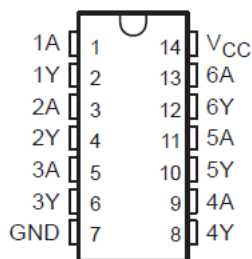
Figure 3-1. CD74ACT14 D or N Package, 14-Pin SOIC or PDIP (Top View)
