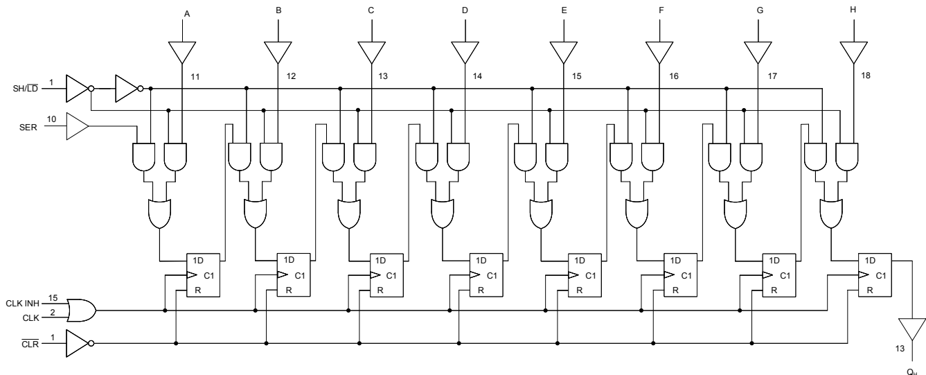
Functional Diagram
