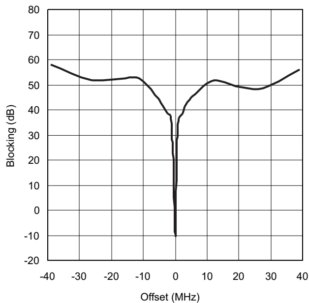
Figure 5-25. Typical Selectivity at 250-kBaud Data Rate
