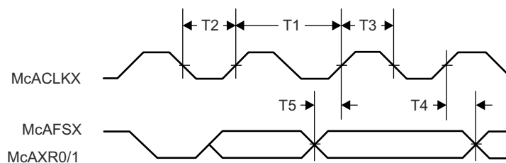
Figure 7-11. I2S Receive Mode Timing Diagram
