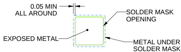
SIGNAL PADS DETAIL
