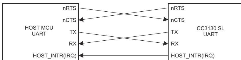
Figure 7-18. 5-Wire UART Topology
