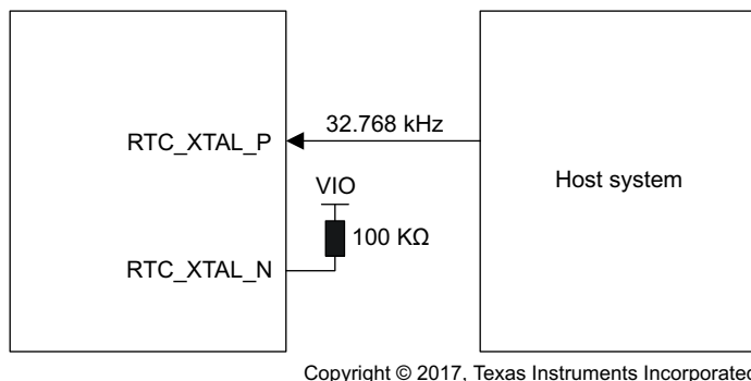
Figure 7-10. External RTC Input
