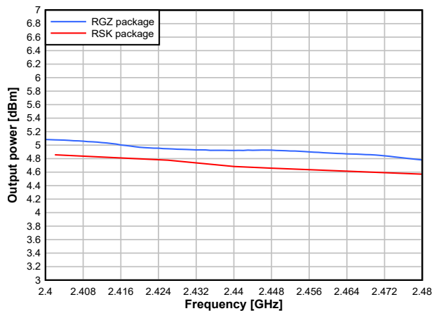
Figure 7-27. Output Power vs. Frequency (BLE 1Mbps, +5dBm)
