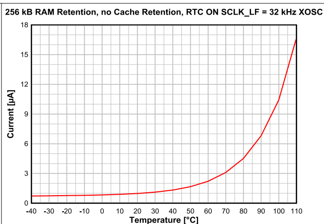
Figure 7-4. Standby Mode (MCU) Current vs. Temperature
