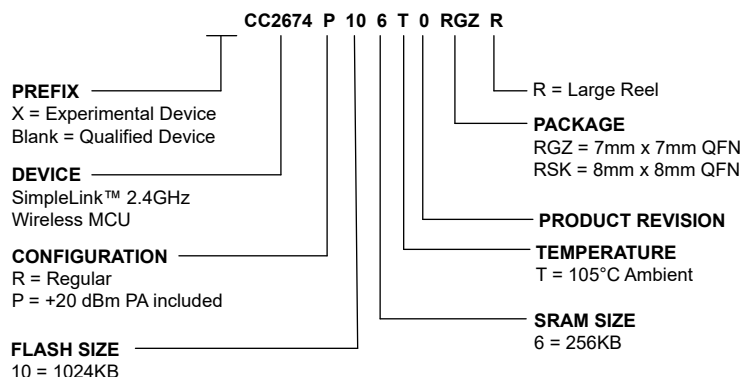
Figure 10-1. Device Nomenclature
