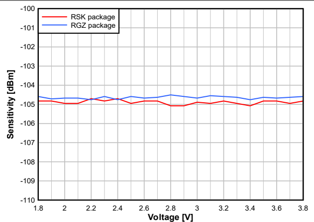
Figure 7-19. Sensitivity vs. Supply Voltage (VDD) (250kbps, 2.44GHz)
