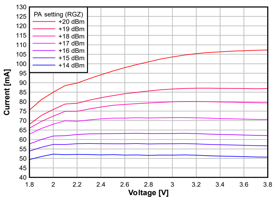
Figure 7-13. TX Current vs. Supply Voltage (VDD) (BLE 1 Mbps, 2.44GHz, +20dBm PA, RGZ package)
