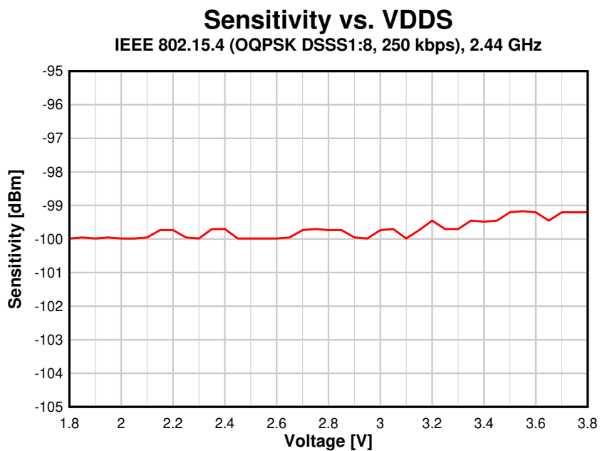
Figure 8-17. Sensitivity vs. Supply Voltage (VDD) IEEE 802.15.4 (OQPSK DSSS1:8, 250 kbps)
