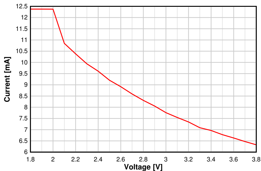
Figure 8-10. TX Current vs. Supply Voltage (VDDS) (BLE 1 Mbps, 2.44 GHz)
