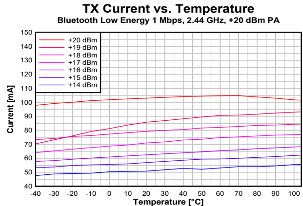
Figure 7-9. TX Current vs. Temperature (Bluetooth Low Energy 1 Mbps, 2.44 GHz, VDD S = 3.3 V)
