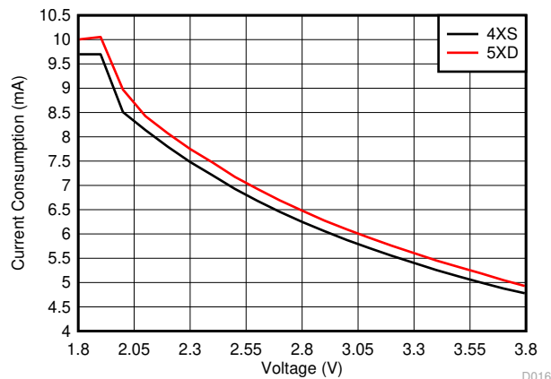
Figure 8-11. RX Mode Current Consumption vs Supply Voltage (VDD5)
