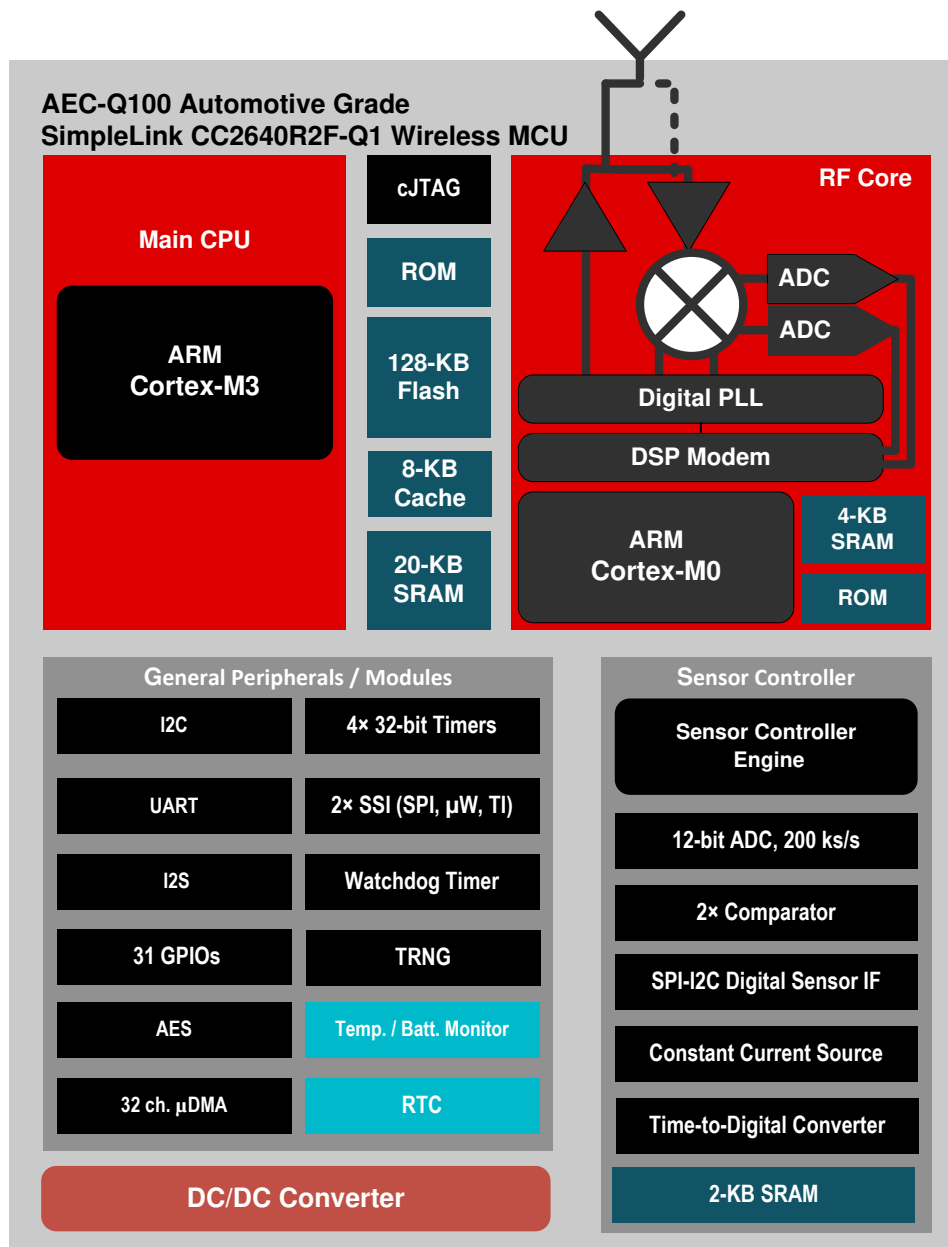
Block Diagram
