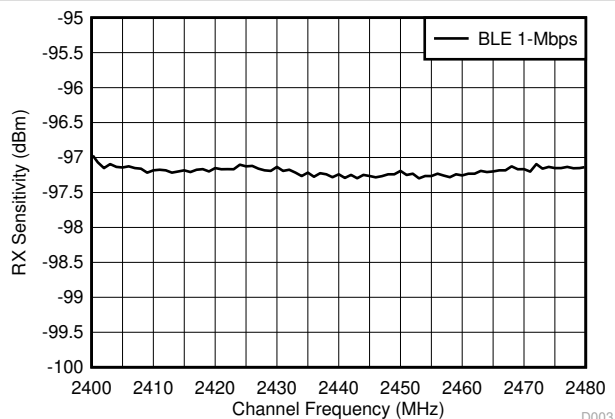
Figure 7-6. Bluetooth Low Energy Sensitivity vs Channel Frequency
