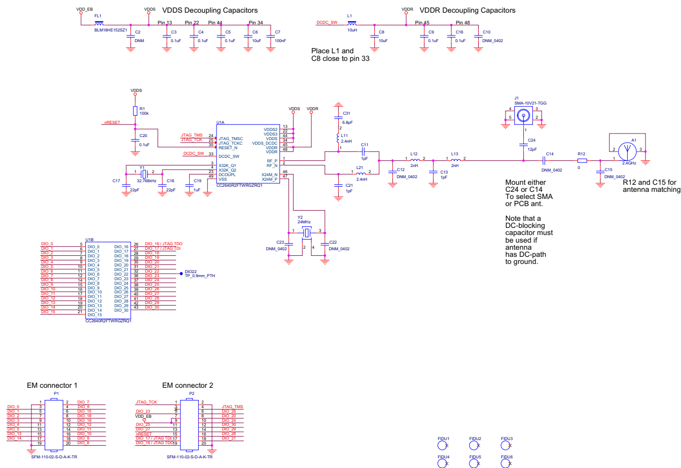
Figure 9-3. 7 × 7 Internal Differential (7ID) Application Circuit
