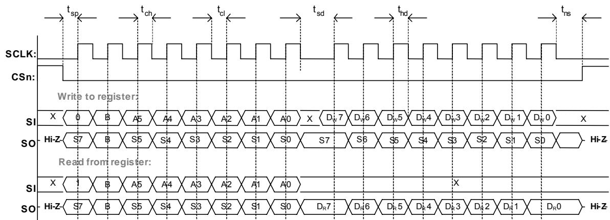
Figure 6: Configuration Registers Write and Read Operations
