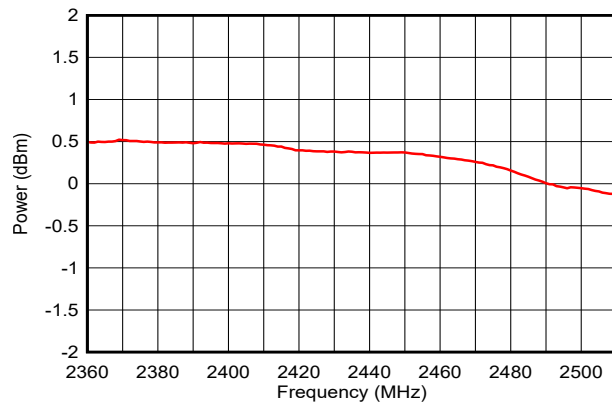
Figure 7-25. Output Power vs. Frequency (BLE 1Mbps, 0dBm)
