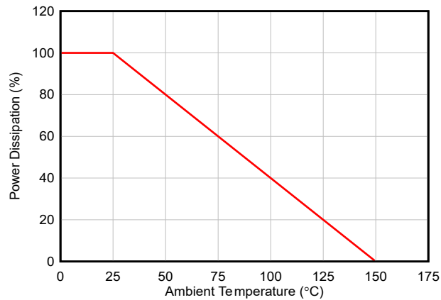
Figure 6-3. Power Derating Curve
