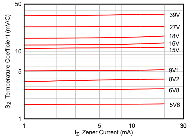
Figure 6-2. Temperature Coefficient
