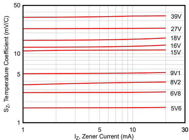
Figure 6-2. Temperature Coefficient
