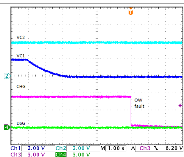
Figure 10-15. OW Fault Protection, Low Voltage—Open Cell1 Connection
