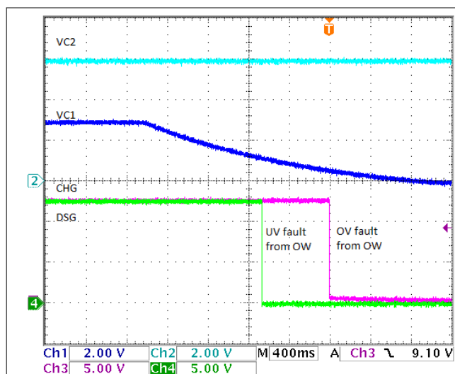
Figure 10-14. OW Fault Protection—Open Cell1 To PCB Connection
