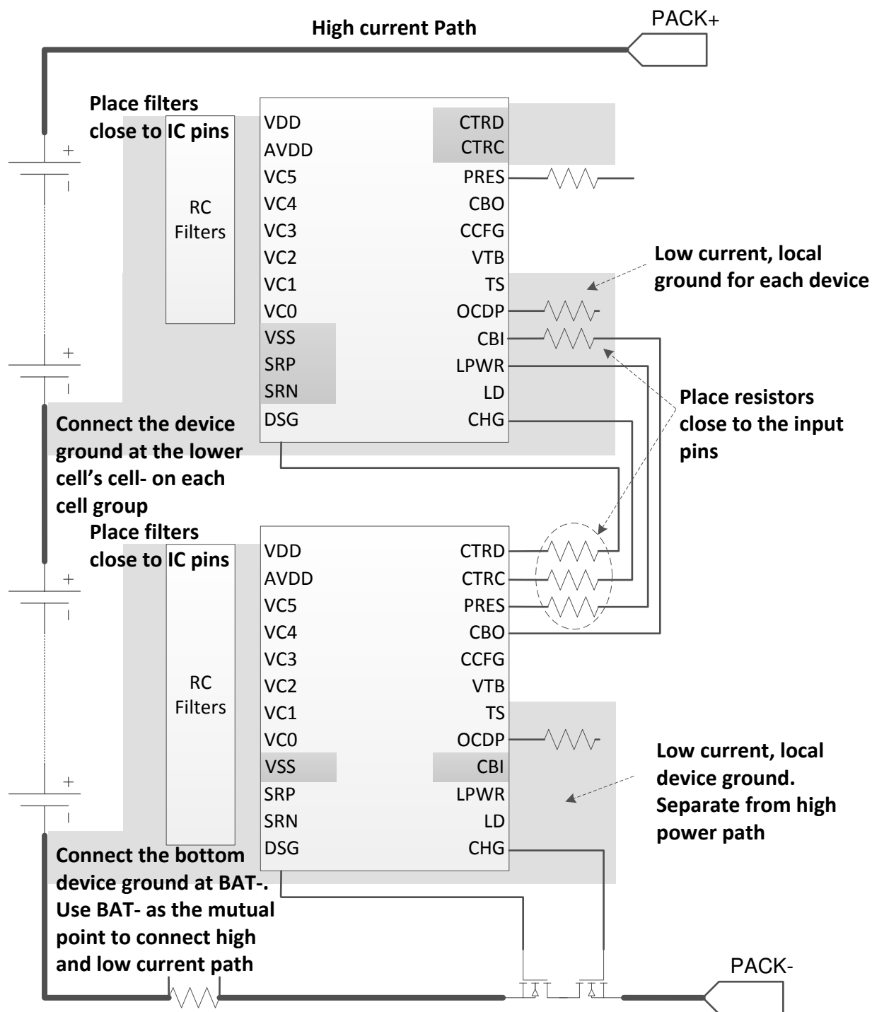
Figure 12-1. Layout Example
