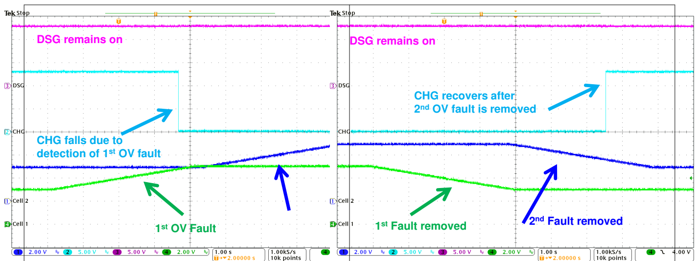
Figure 9-10. OV Fault Protection
