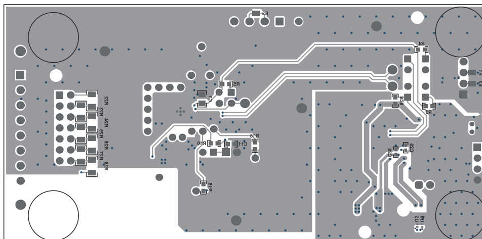
Figure 10-2. BQ77307 Two-Layer Board Layout–Bottom Layer
