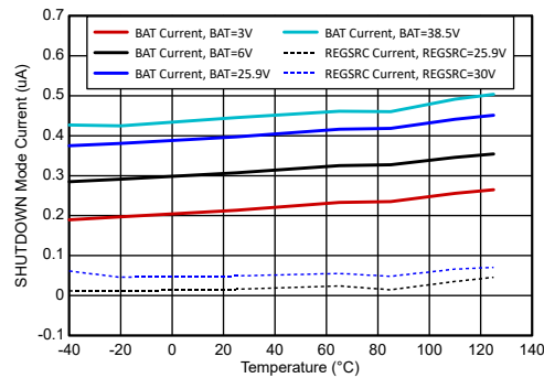
Figure 6-12. Supply Current in SHUTDOWN Mode vs. Temperature
