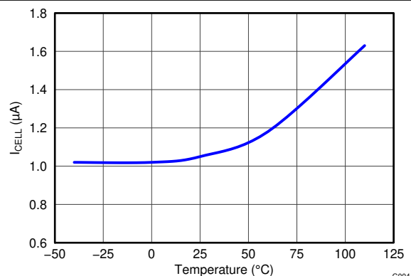
Figure 9-6. I_{CELL} vs. Temperature at V_{CELL} = 9.2 V
