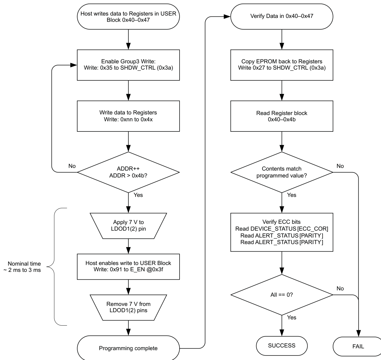
Figure 23. EPROM Programming
