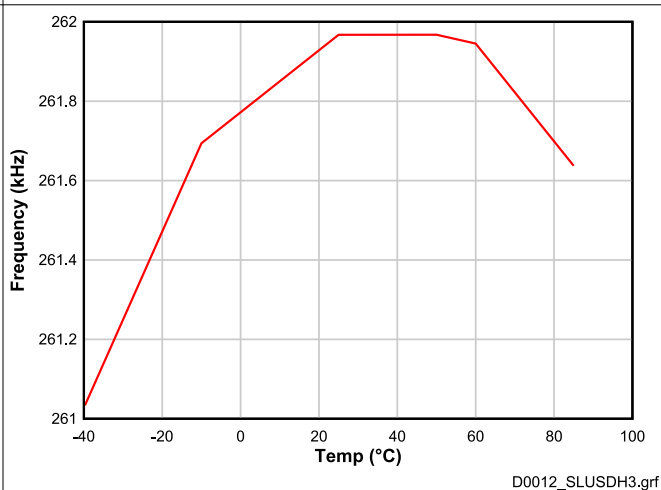
Figure 6-7. Low Frequency Oscillator (LFO) Accuracy vs. Temperature
