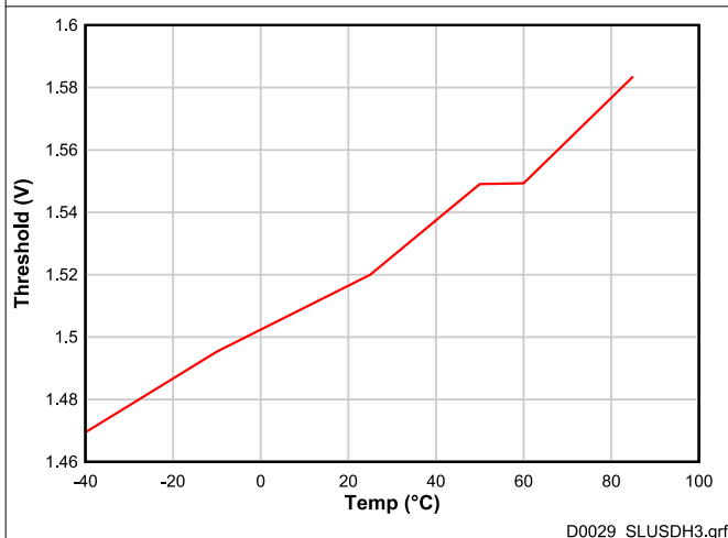
Figure 6-18. LD Wake Voltage vs. Temperature
