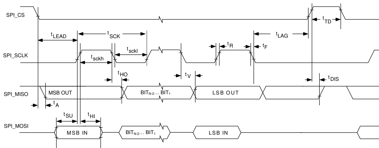
Figure 6-2. SPI Communications Interface Timing
