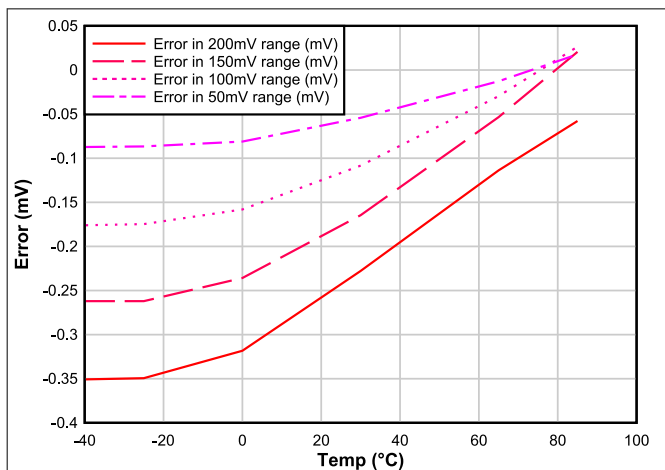
Figure 6-4. Current Measurement Error vs. Temperature
