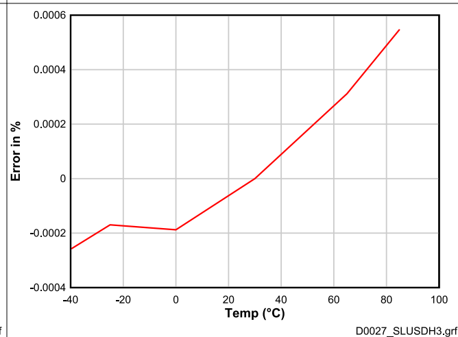
Error calculated as percentage of nominal gain across \pm 200 -mV input range Figure 6-17. Coulomb Counter Gain Error vs. Temperature
