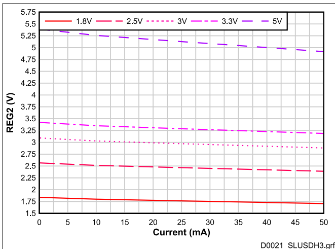
Figure 6-14. REG2 Voltage vs. Load at 25°C
