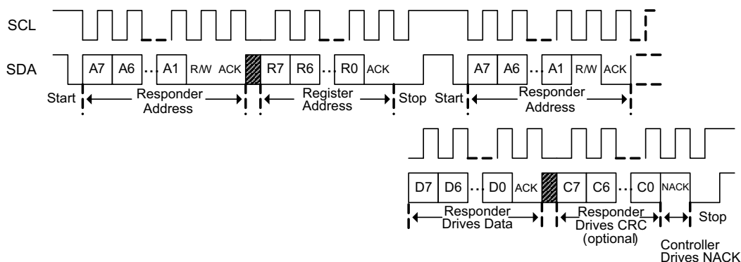
Figure 7-8. I²C Read Without Repeated Start
