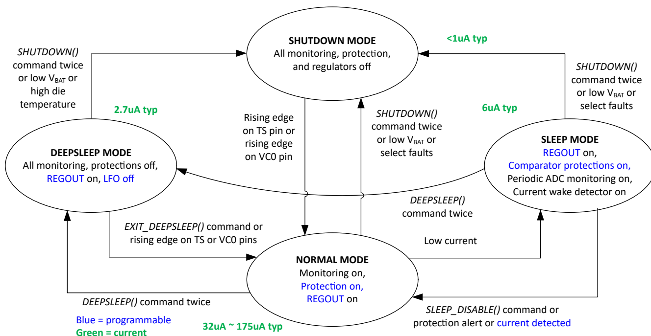
Figure 7-6. BQ76905 Operational Power Modes
