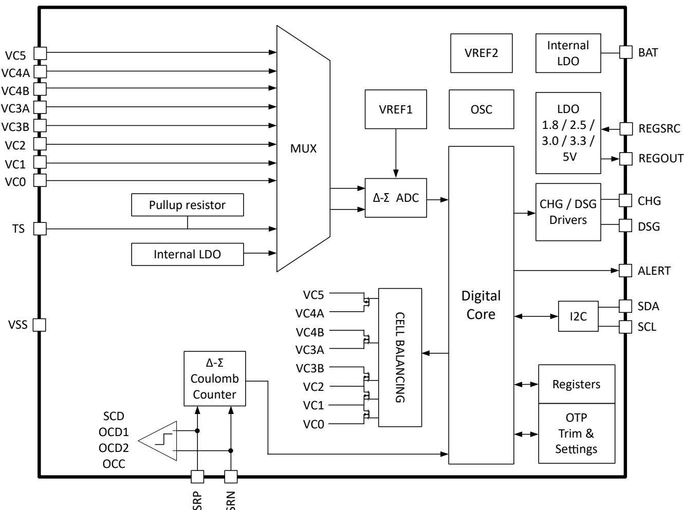
Figure 7-1. BQ76905 Block Diagram
