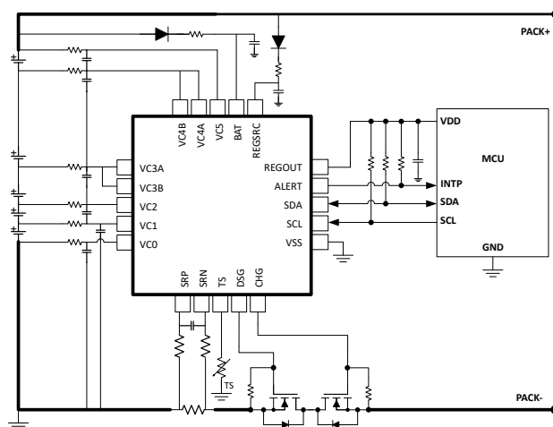
Figure 3-1. Simplified Schematic
