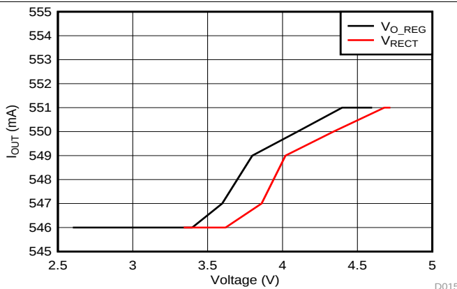
Figure 43. Dynamic Regulation on a WPC TX
