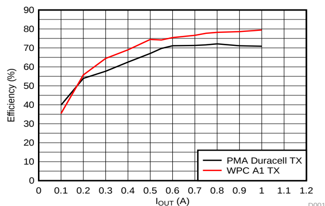
Dual Mode Efficiency 5-V Out
