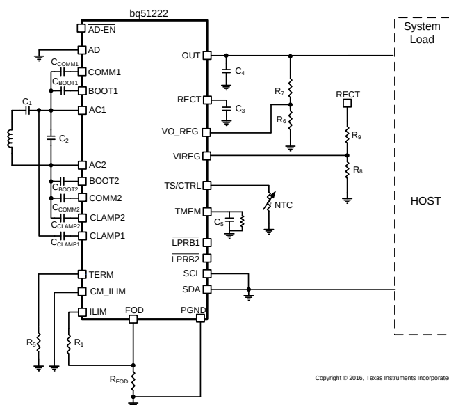
Simplified Schematic
