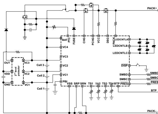
Simplified Schematic
