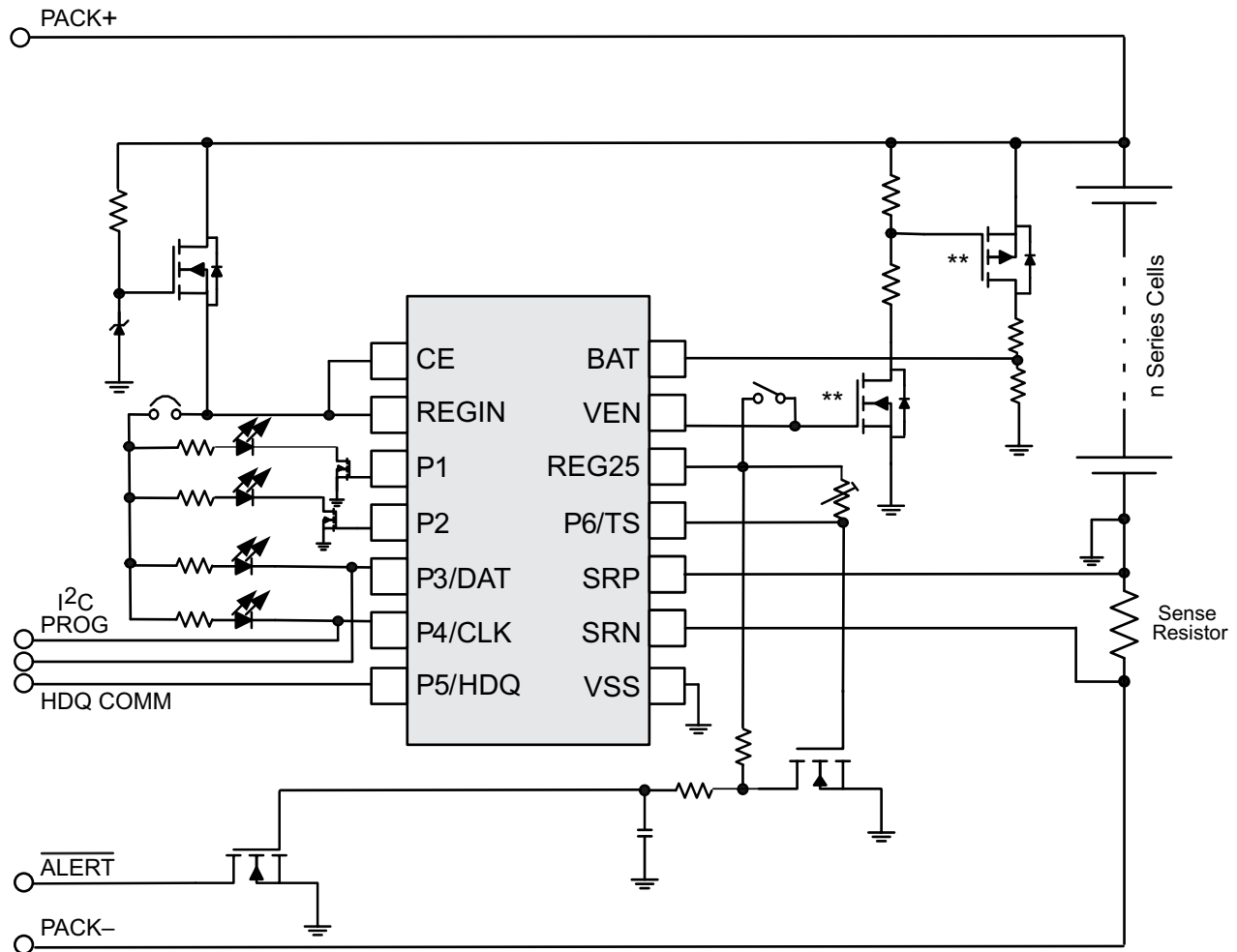
Figure 2. bq34z110 Typical Implementation
