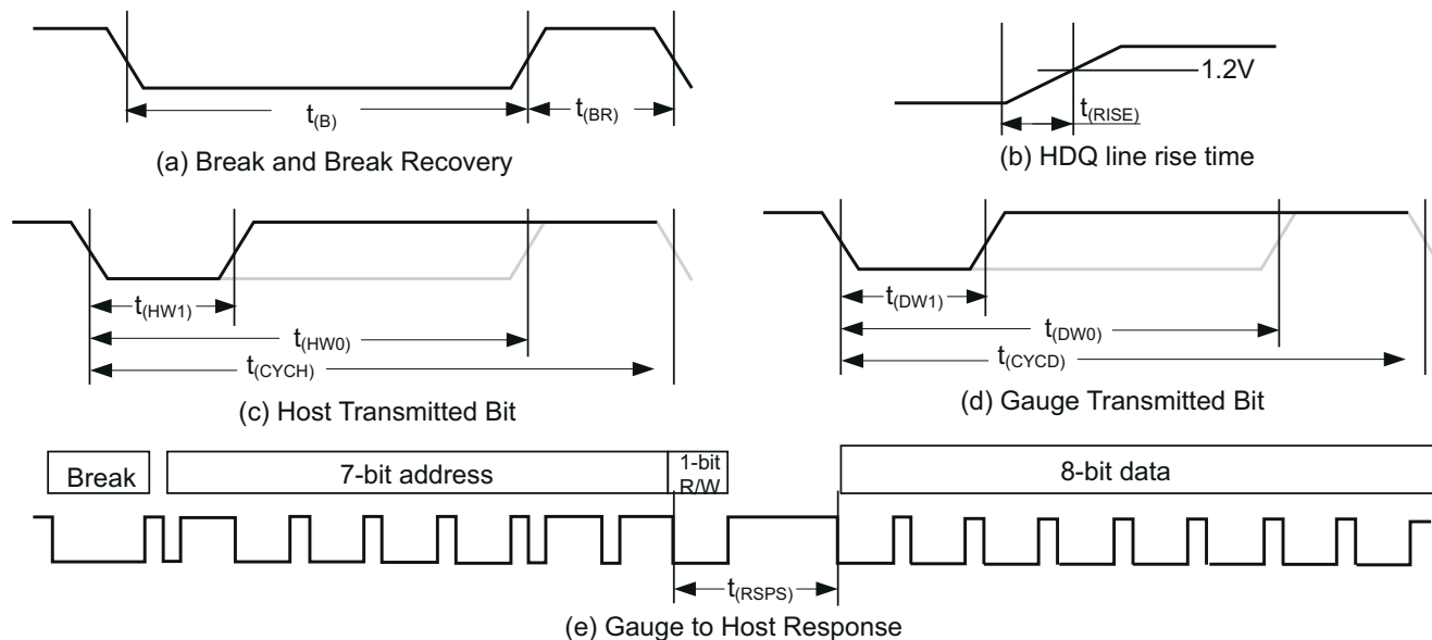
Figure 6-1. Timing Diagrams
