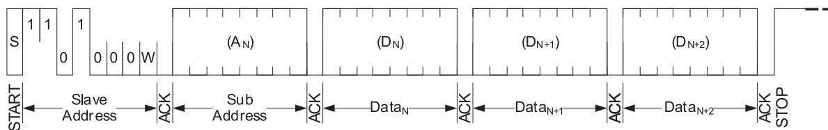
Figure 7. I²C Write Mode
