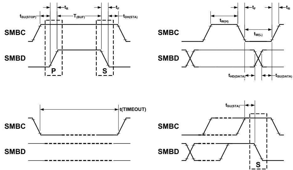
Figure 6. SMBus Timing Diagram
