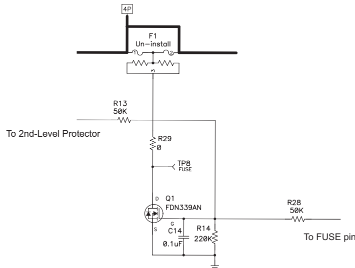
Figure 16. FUSE Circuit
