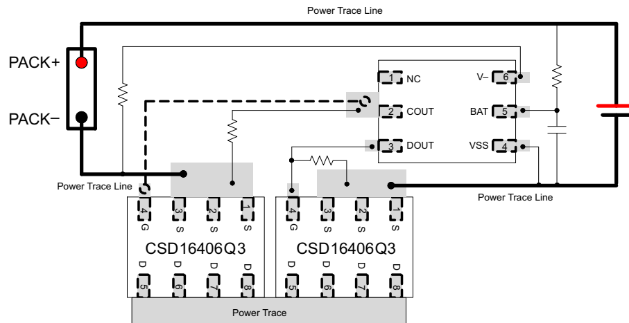
Figure 9-8. BQ2970 Board Layout
