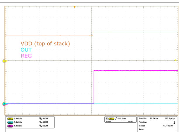
Figure 8-7. Undervoltage Recovery to Re-enable the Regulator
