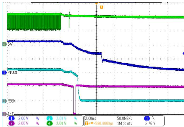
Figure 59. Adapter Removal
