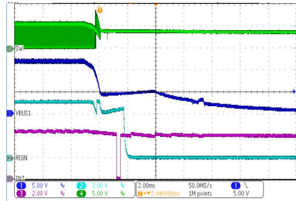
Figure 60. Adapter Removal
