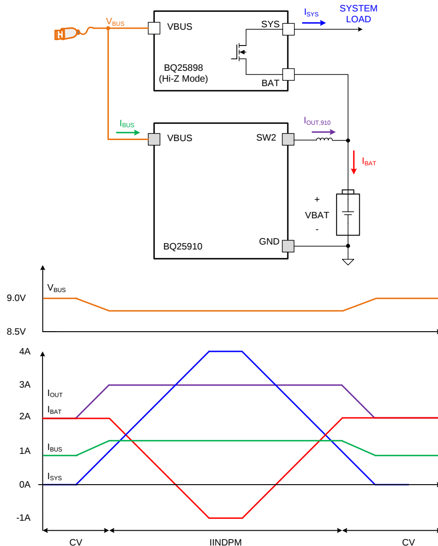
Figure 20. DPM Response
