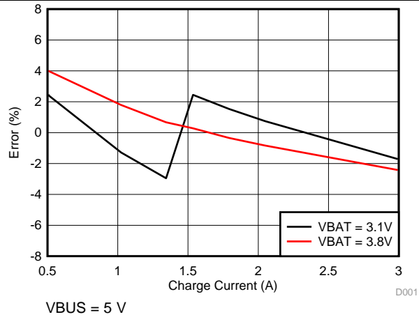
Figure 3. Charge Current Accuracy vs Charge Current I 2 C Setting
