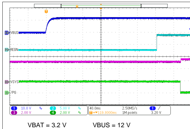
Figure 47. Power Up with Charge Disabled
