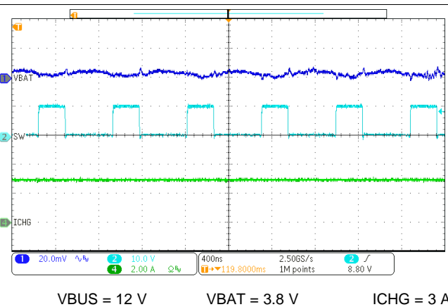
Figure 50. PWM Switching Waveform
