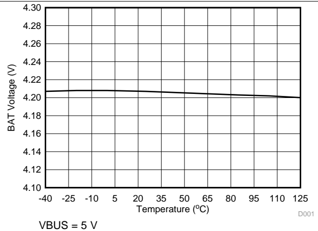
Figure 6. BAT Voltage vs Temperature
