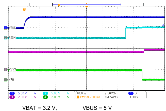
Figure 41. Power Up with Charge Disabled
