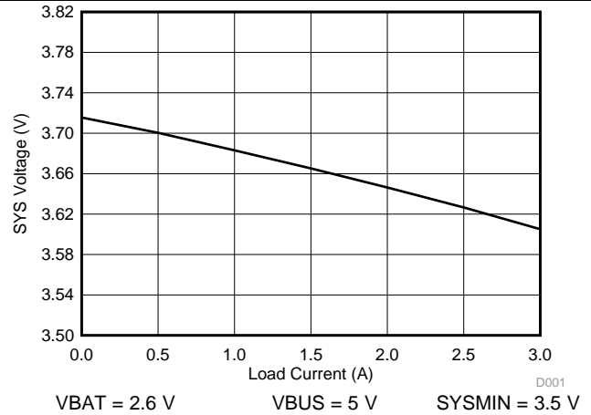
Figure 4. SYS Voltage Regulation vs System Load Current
