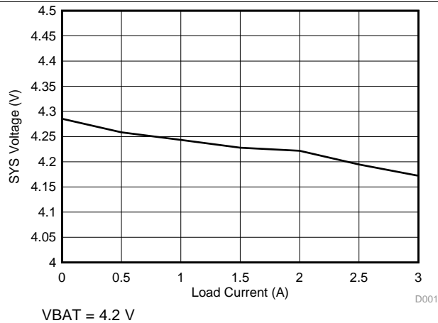
Figure 5. SYS Voltage Regulation vs System Load Current
