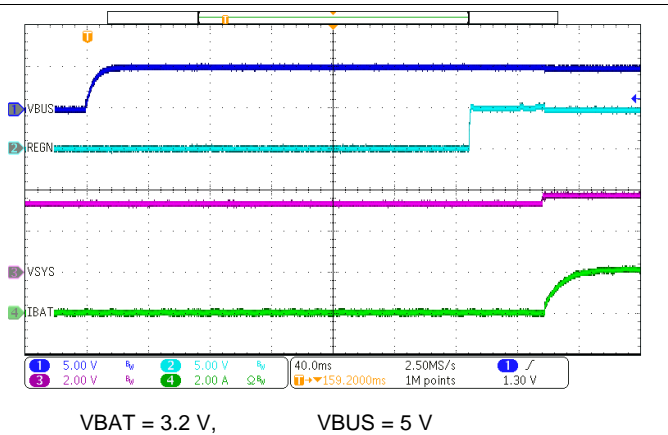
Figure 42. Power Up with Charge Enabled
