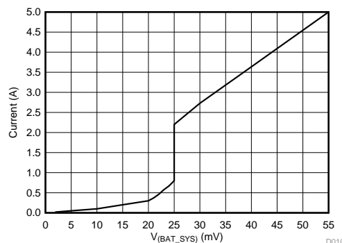
Figure 11. BATFET V-I Curve
