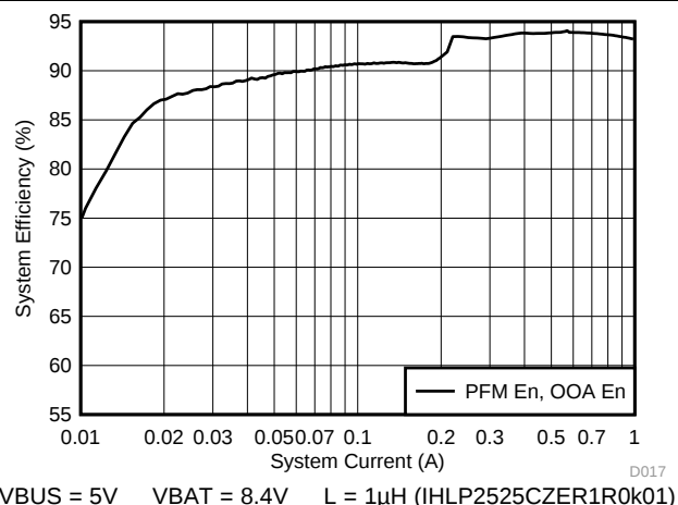
Figure 4. System Efficiency vs. System Current
