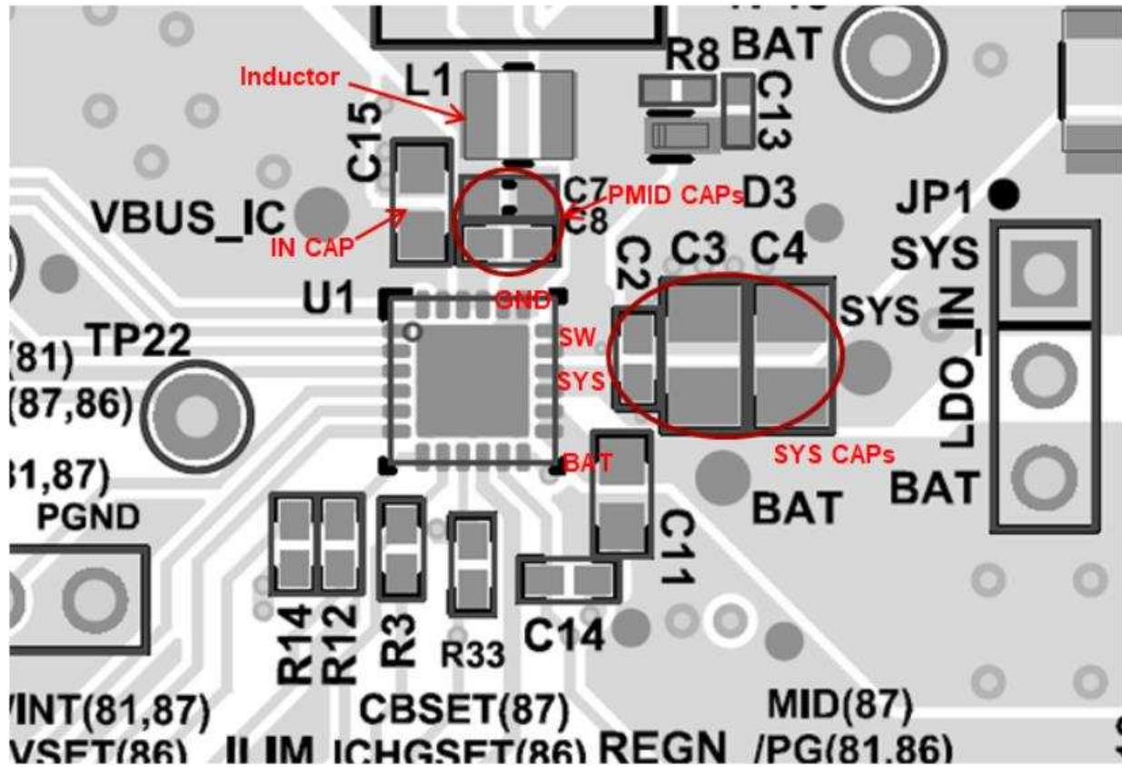
Figure 35. PCB Layout Example
