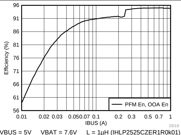
Figure 6. OTG Efficiency vs. VBUS Output Current
