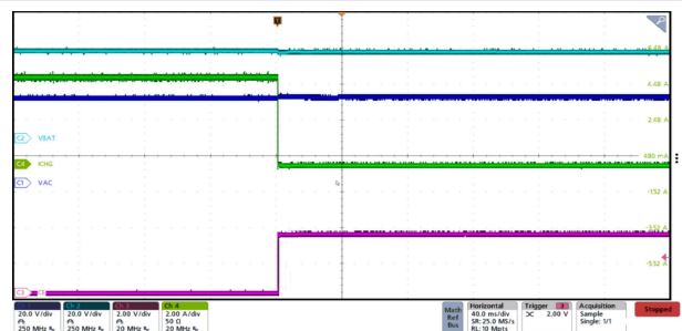
Figure 8-6. Charge Disable via I 2 C with 5-A ICHG
