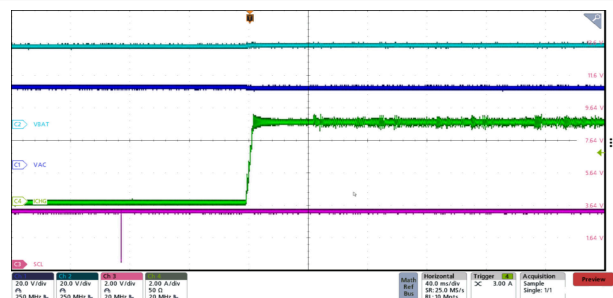
Figure 8-5. Charge Enable via I 2 C with 5-A ICHG
