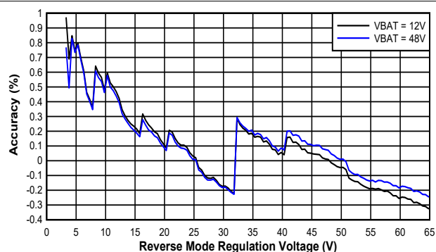
Figure 6-13. Reverse Mode Output Voltage Accuracy vs VAC_REV Setting
