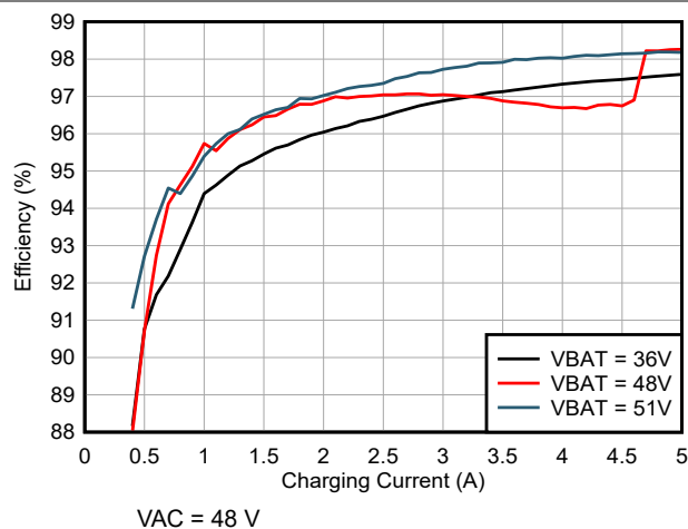
Figure 6-2. Charge Efficiency vs Charge Current
