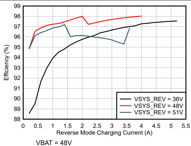
Figure 6-12. Reverse Mode Efficiency (12s Li-Ion battery configuration)
