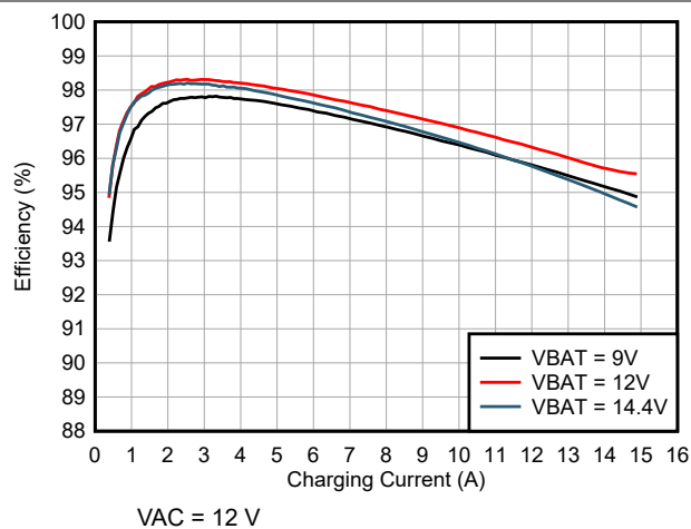
Figure 6-1. Charge Efficiency vs Charge Current (4s LiFePO4 battery configuration)
