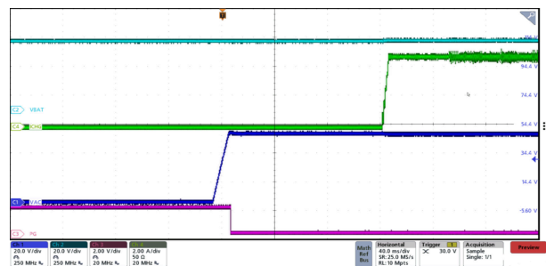
Figure 8-3. VAC Plug-In Power Up with 5-A ICHG
