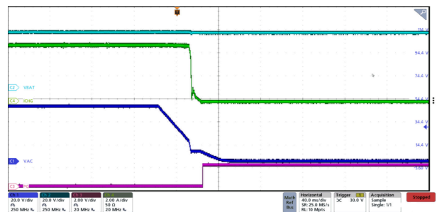
Figure 8-4. VAC Un-plug Power Down with 5-A ICHG
