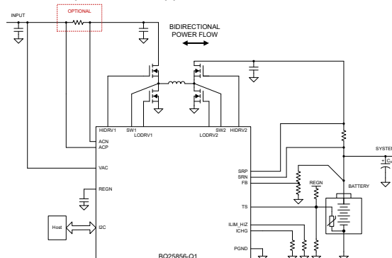
Simplified Schematic
