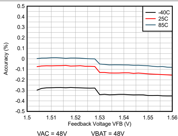
Figure 6-4. Feedback Voltage Accuracy (at different temperatures)
