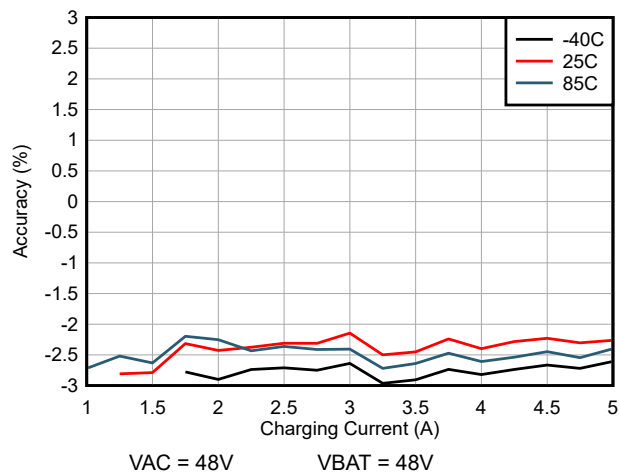
Figure 6-6. Charge Current Accuracy (at different temperatures)
