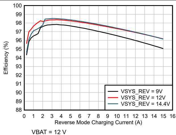
Figure 6-11. Reverse Mode Efficiency (4s LiFePO4 battery configuration)
