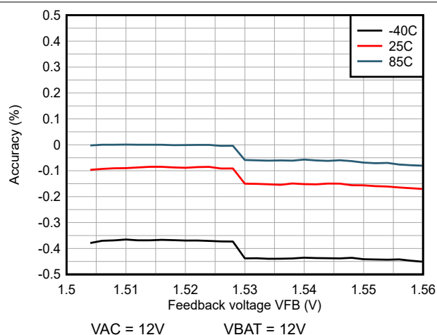
Figure 6-3. Feedback Voltage Accuracy (at different temperatures)
