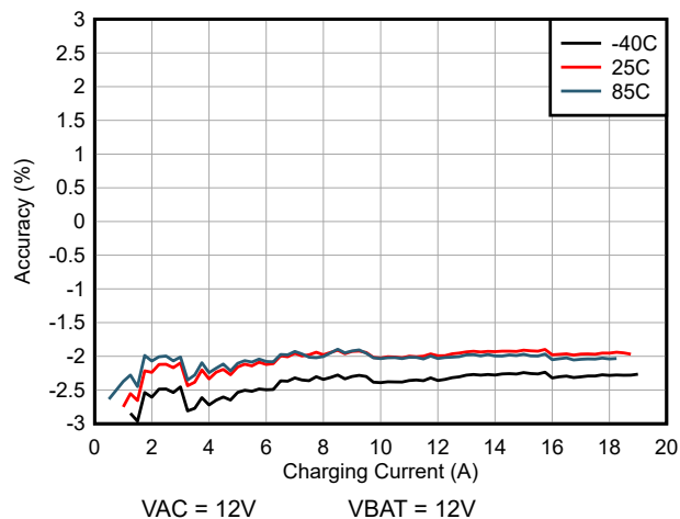
Figure 6-5. Charge Current Accuracy (at different temperatures)
